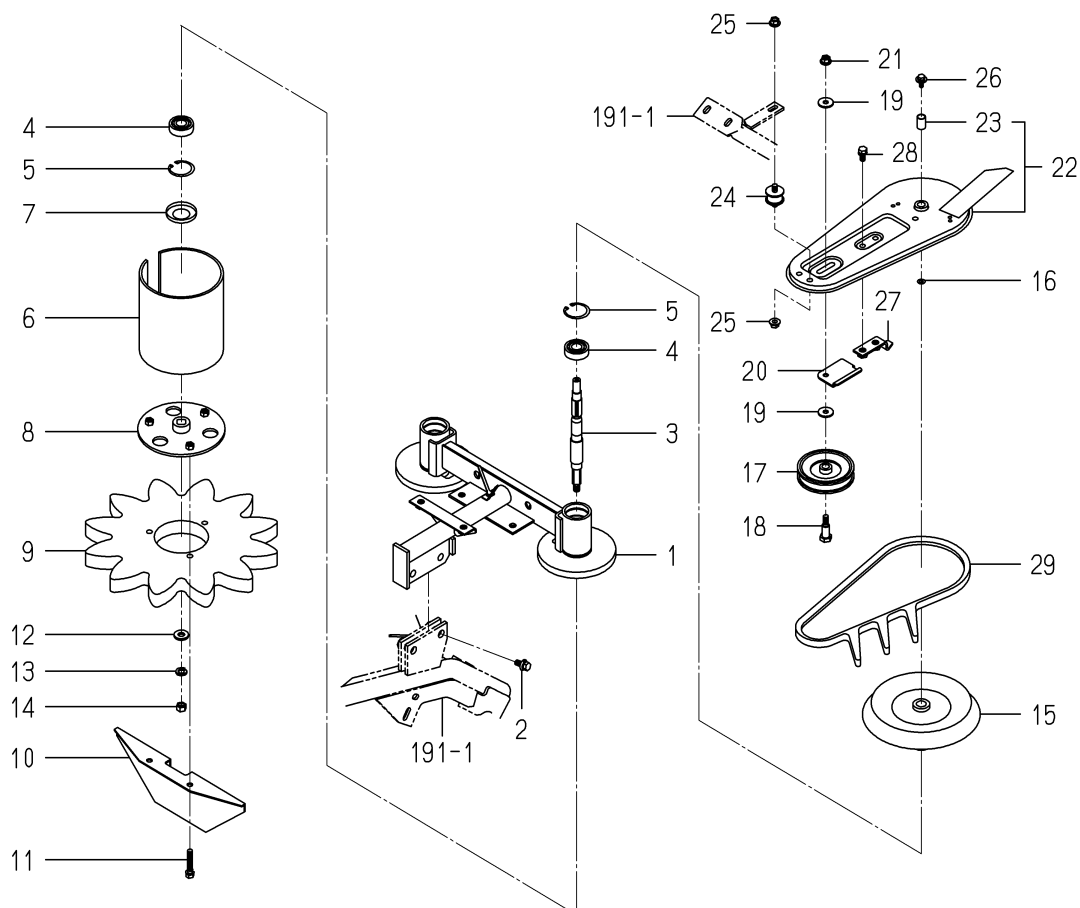
FIG.143 レイクアツプ(RH/3RD, 2ND)関係(図1/2)
