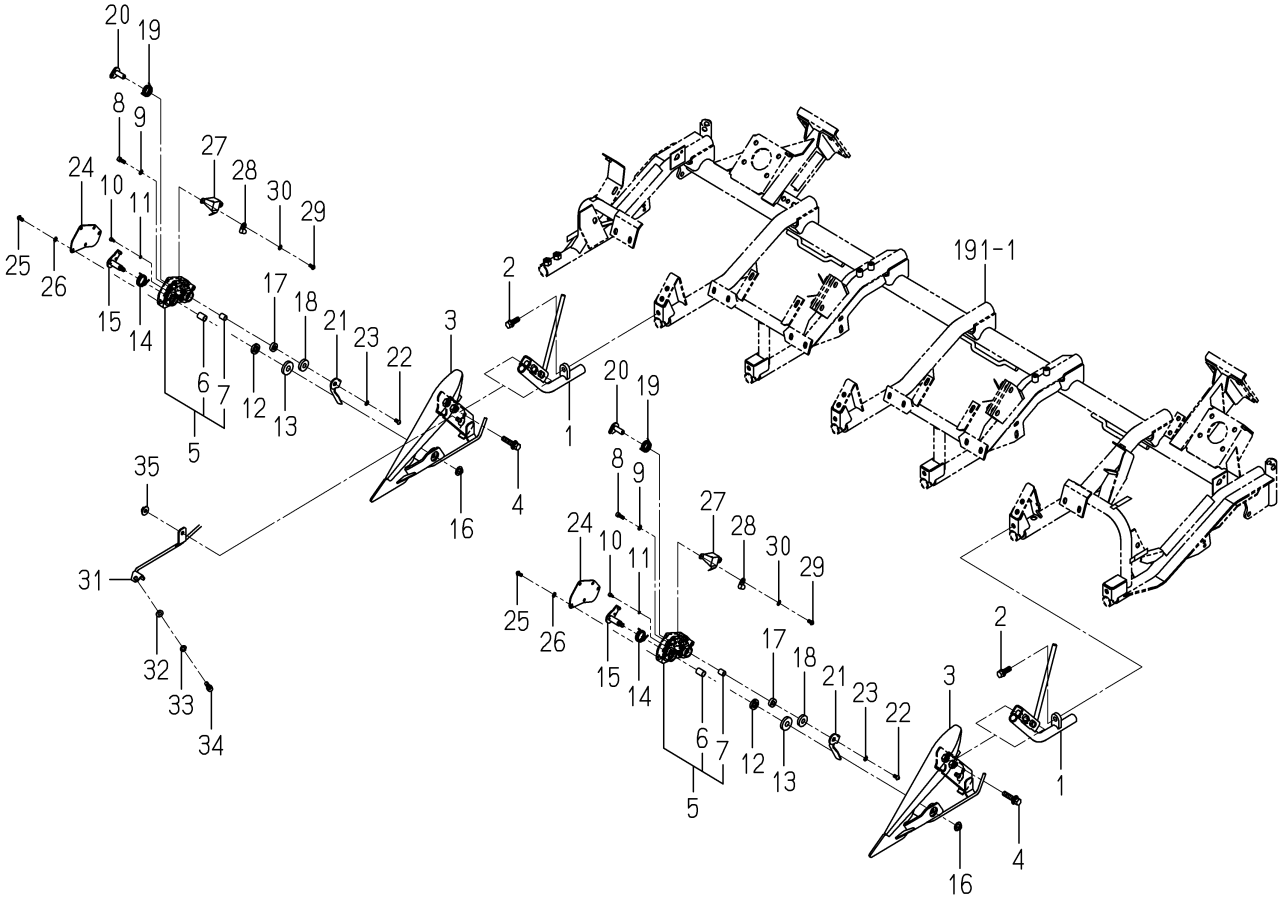
FIG.116 デバイダ(LH／2ND, RH／2ND)関係
